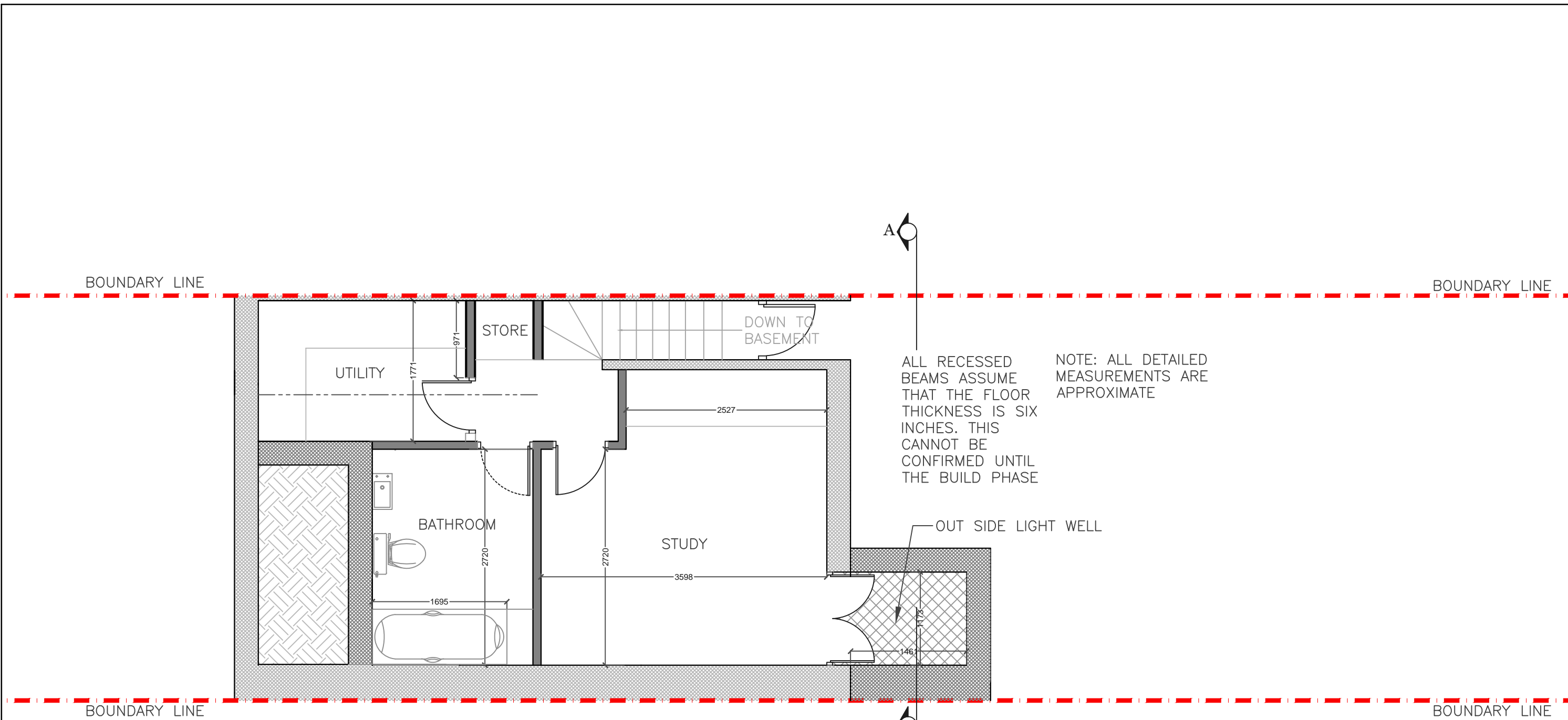
PROPOSED BASEMENT PLAN 1:50
